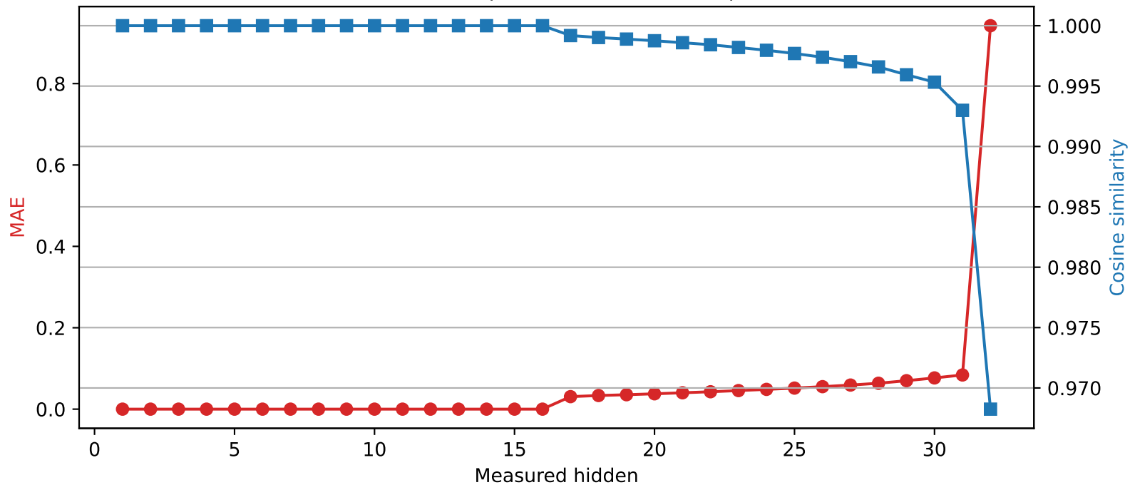
Mistral-7B-Instruct-v0.3 | Quantized layer 16 | float32 → int2
