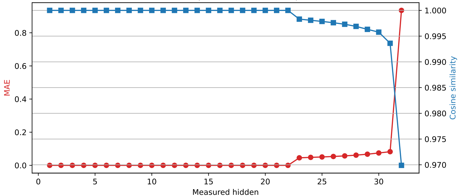
Mistral-7B-Instruct-v0.3 | Quantized layer 22 | float32 → int2
