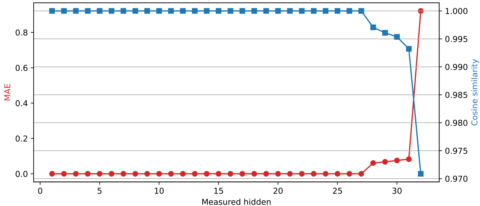
Mistral-7B-Instruct-v0.3 | Quantized layer 27 | float32 → int2
