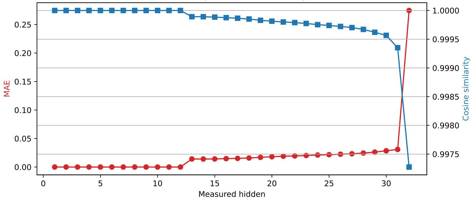
Mistral-7B-Instruct-v0.3 | Quantized layer 12 | float32 → int2
