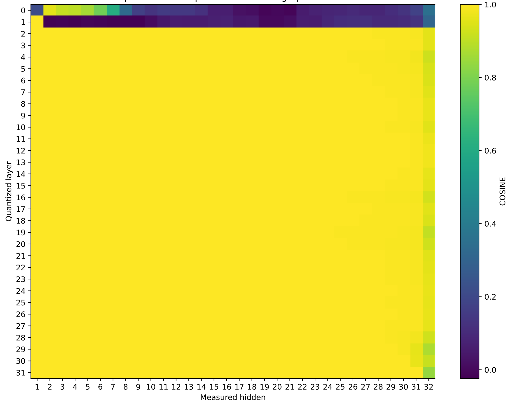
Mistral-7B-Instruct-v0.3 Prompt 1: cos sim representation damage | float64 → int2
