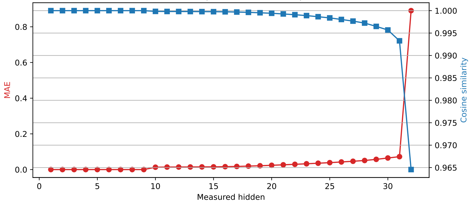
Mistral-7B-Instruct-v0.3 | Quantized layer 9 | float64 → int2
