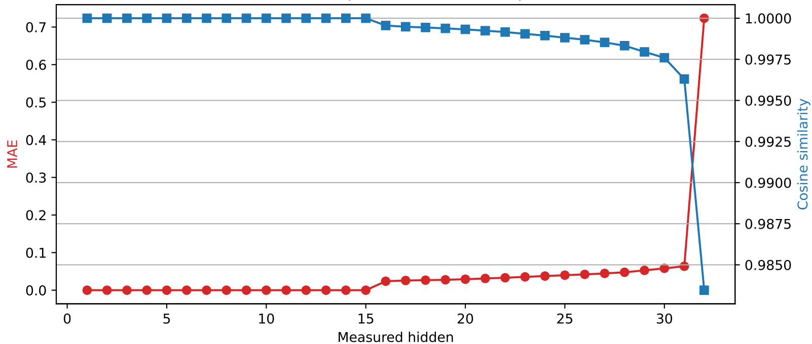
Mistral-7B-Instruct-v0.3 | Quantized layer 15 | float64 → int2
