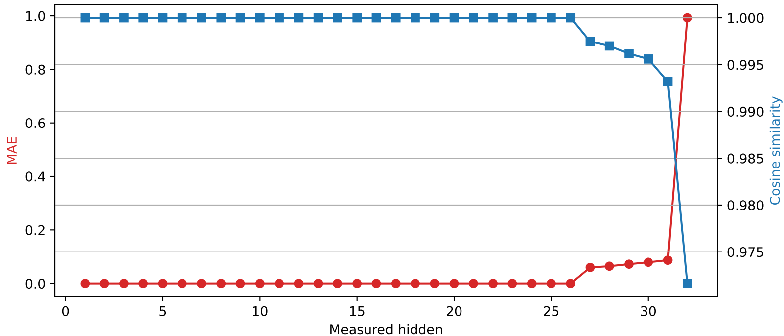
Mistral-7B-Instruct-v0.3 | Quantized layer 26 | float64 → int2
