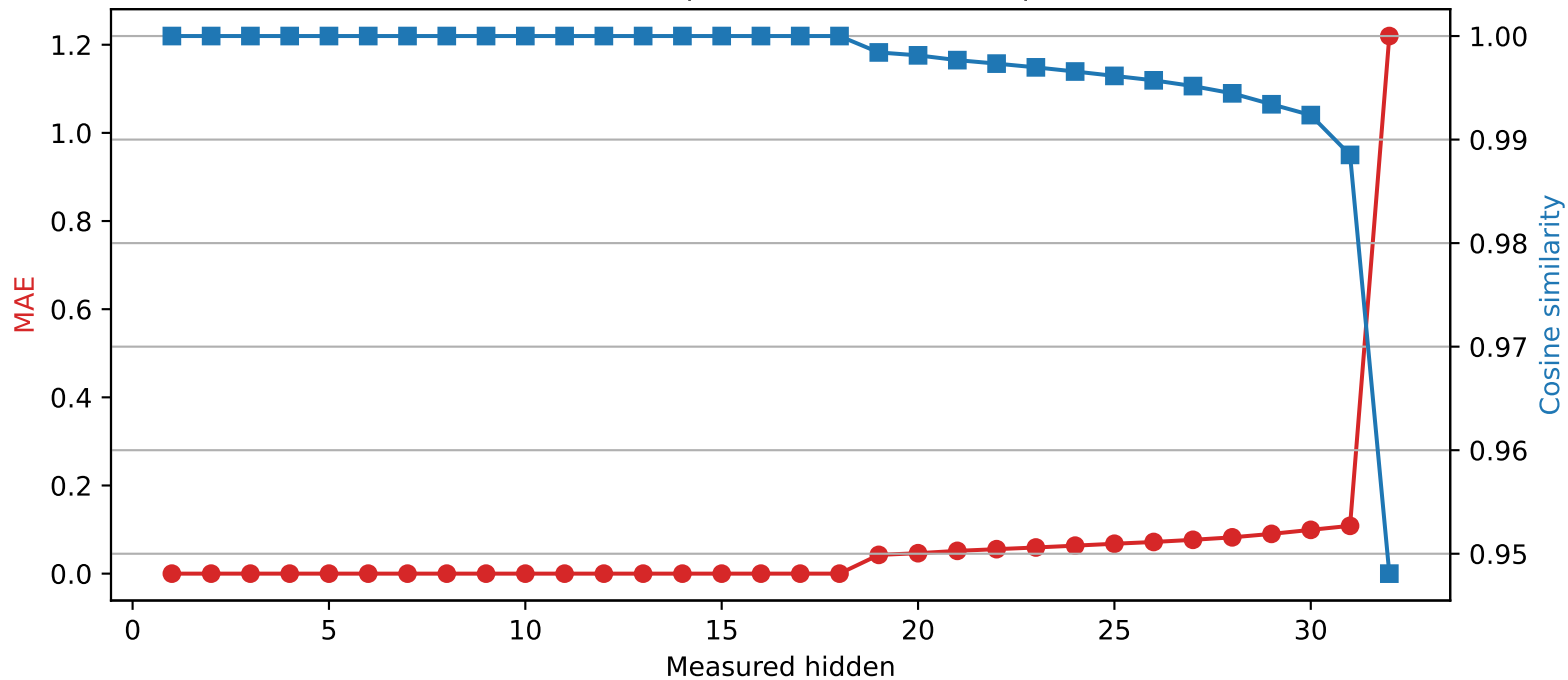
Mistral-7B-Instruct-v0.3 | Quantized layer 18 | float64 → int2
