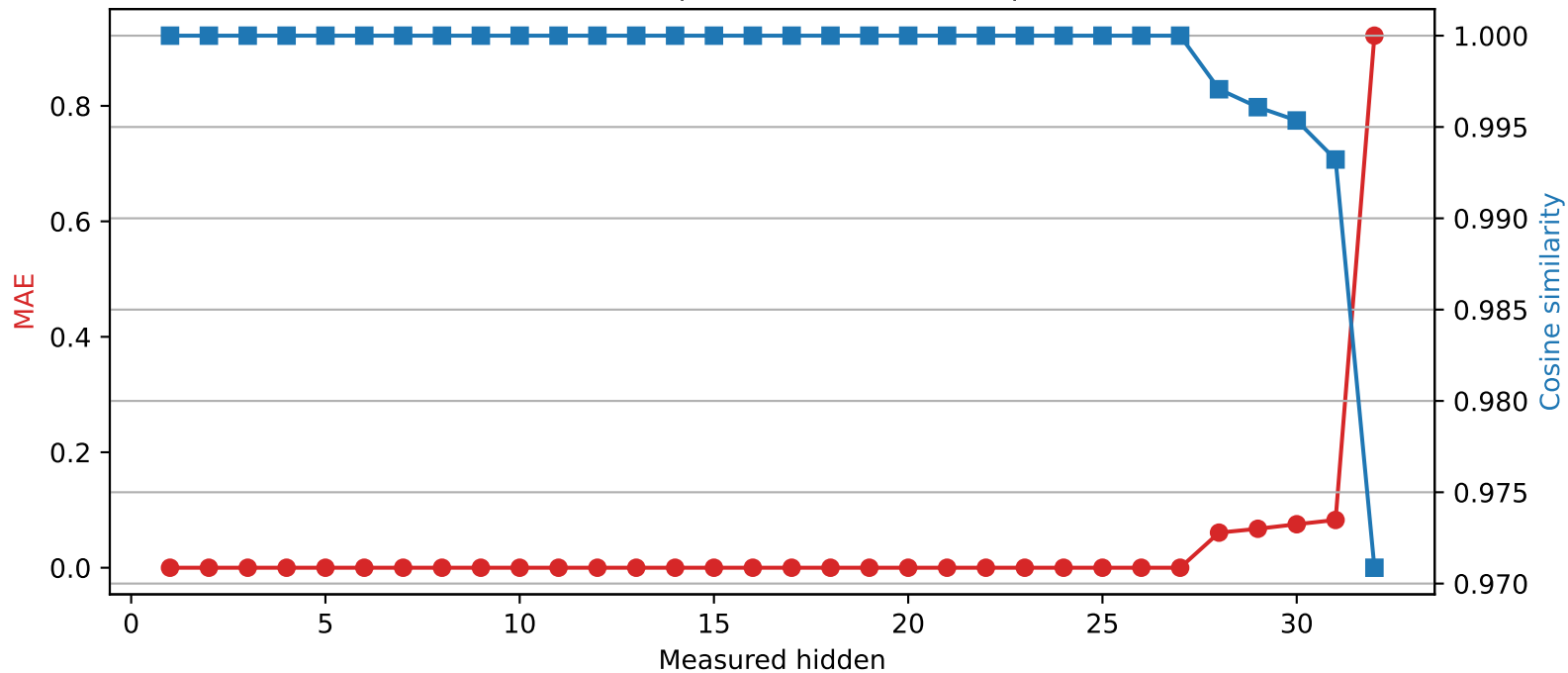
Mistral-7B-Instruct-v0.3 | Quantized layer 27 | float64 → int2
