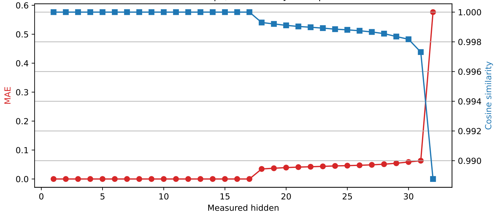
Mistral-7B-Instruct-v0.3 | Quantized layer 17 | float64 \rightarrow int2
