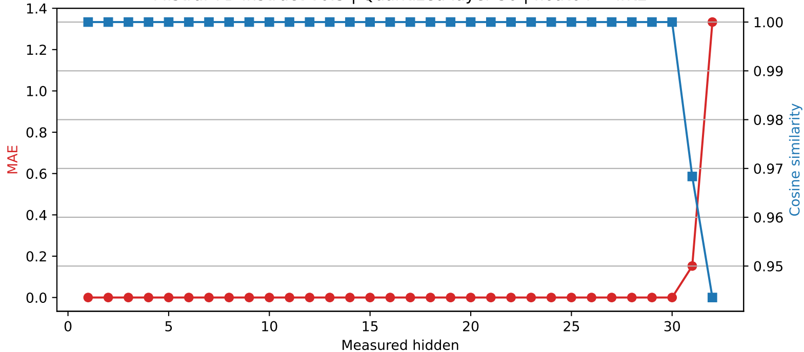
Mistral-7B-Instruct-v0.3 | Quantized layer 30 | float64 → int2
