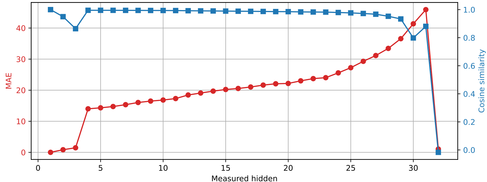
SmolLM2-360M | Prompt 0 Spared layer 0 | Unquantized vs hybrid
