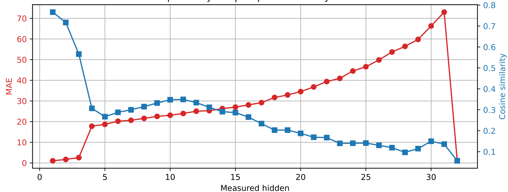
SmolLM2-360M | Prompt 0 Spared layer 6 | Unquantized vs hybrid
