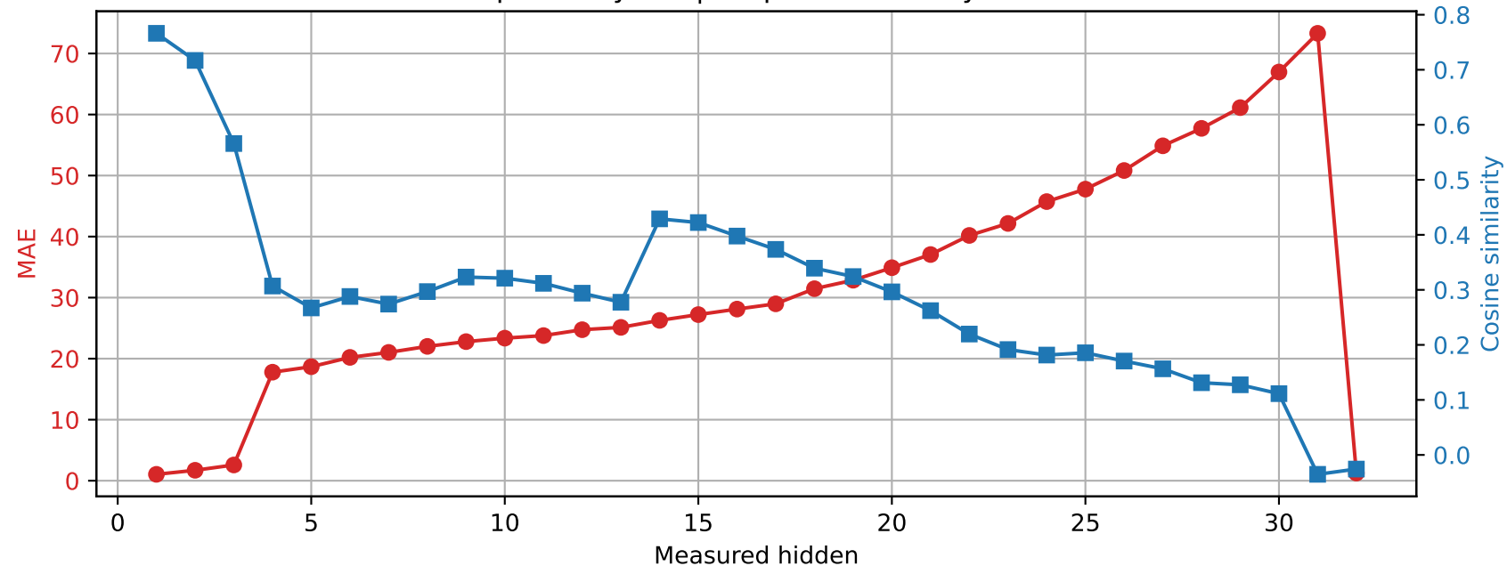
SmolLM2-360M | Prompt 0 Spared layer 9 | Unquantized vs hybrid
