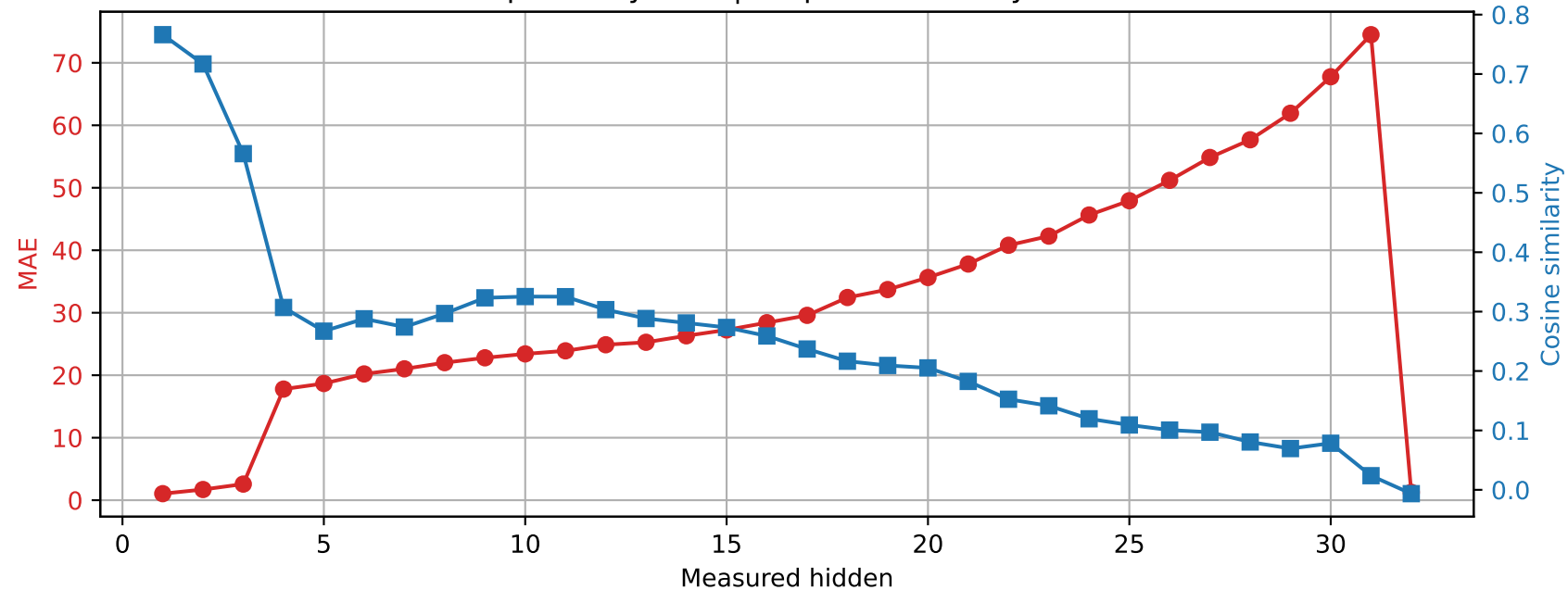
SmolLM2-360M | Prompt 0 Spared layer 22 | Unquantized vs hybrid
