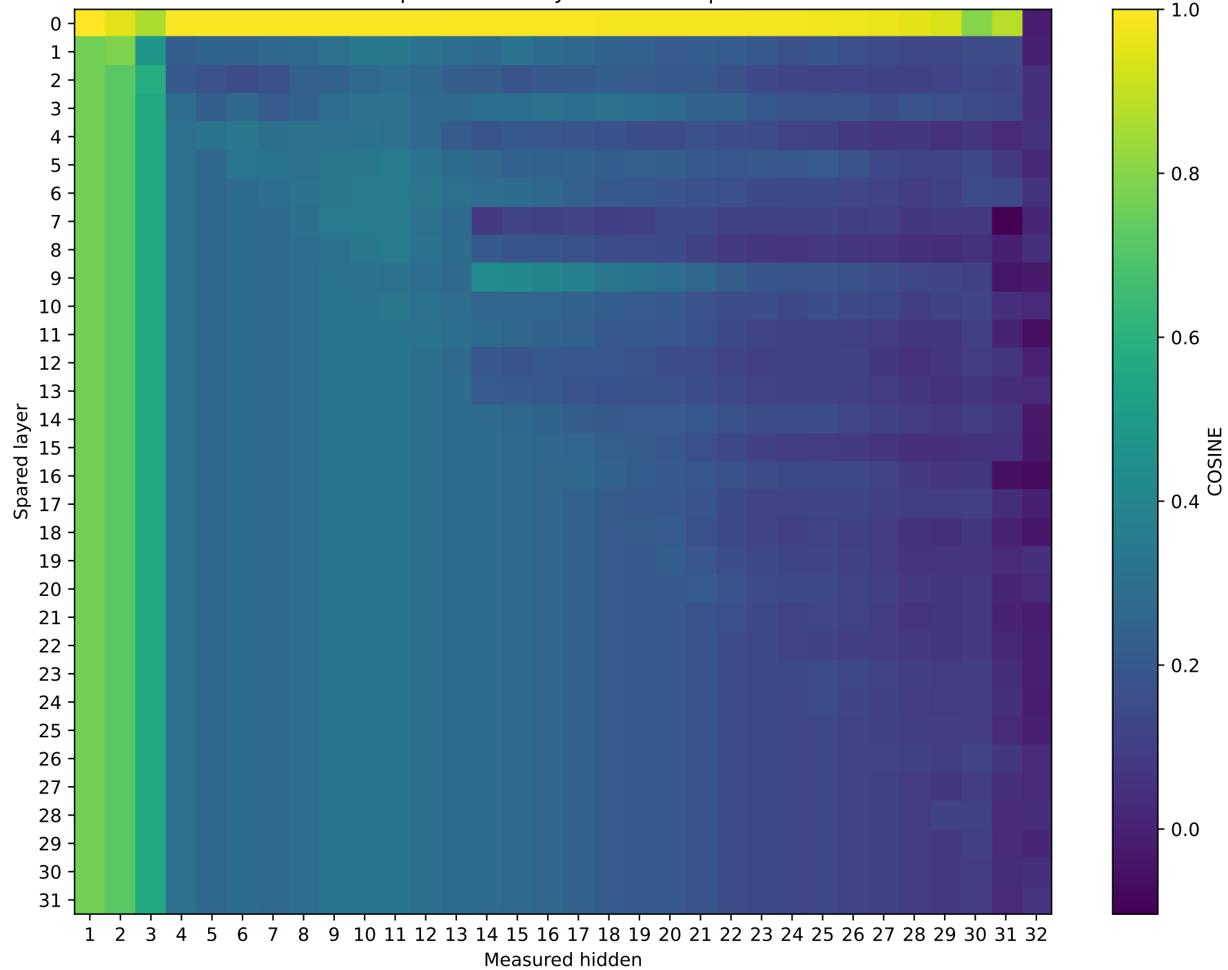
SmolLM2-360M | Prompt 0 Unquantized vs hybrid cos sim | int4
