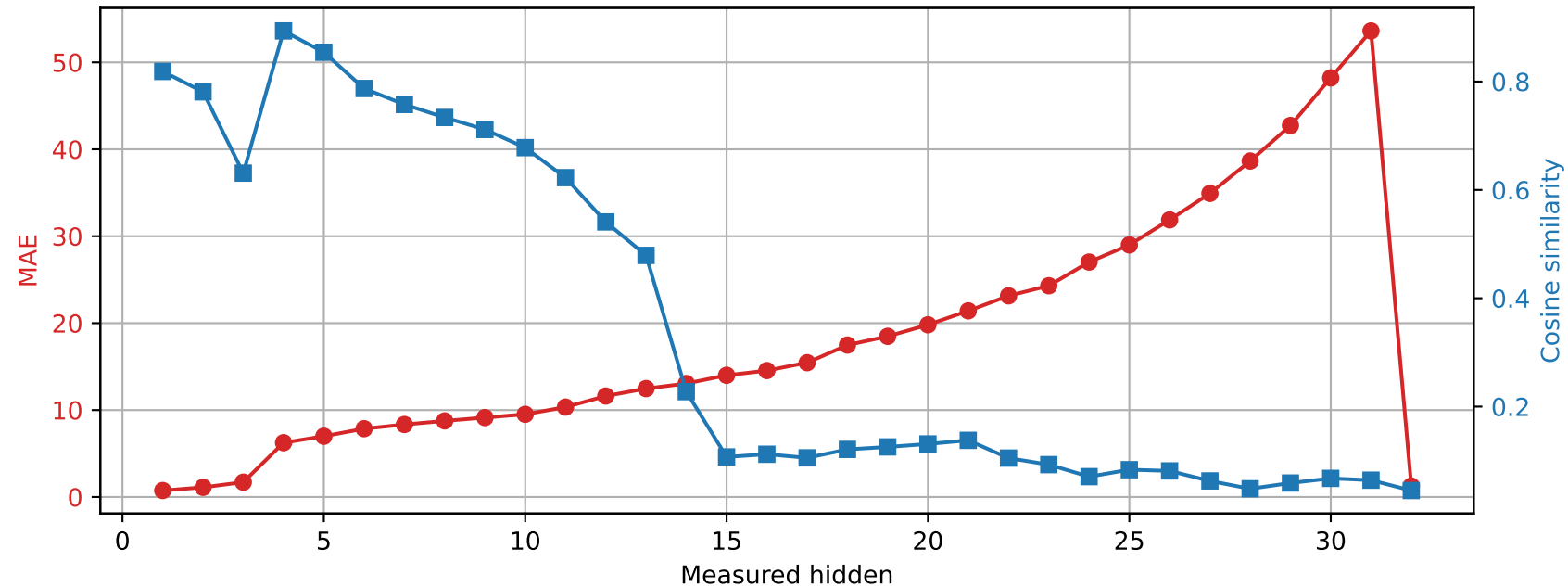
SmolLM2-360M | Prompt 1 Unquantized vs quantized int4
