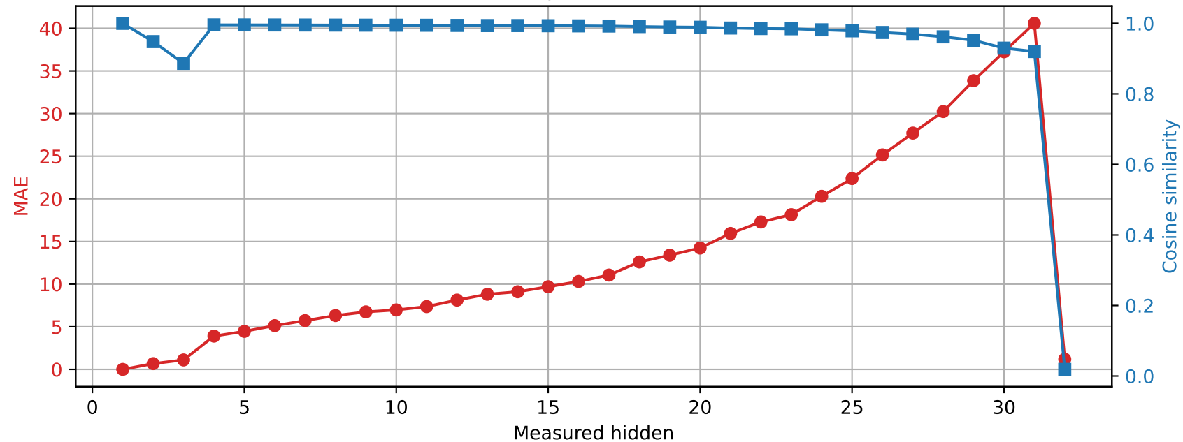
SmolLM2-360M | Prompt 1 Spared layer 0 | Unquantized vs hybrid
