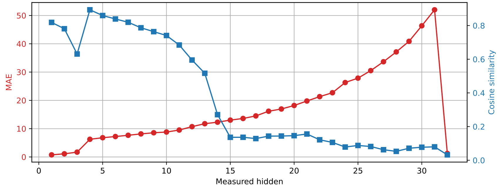
SmolLM2-360M | Prompt 1 Spared layer 4 | Unquantized vs hybrid
