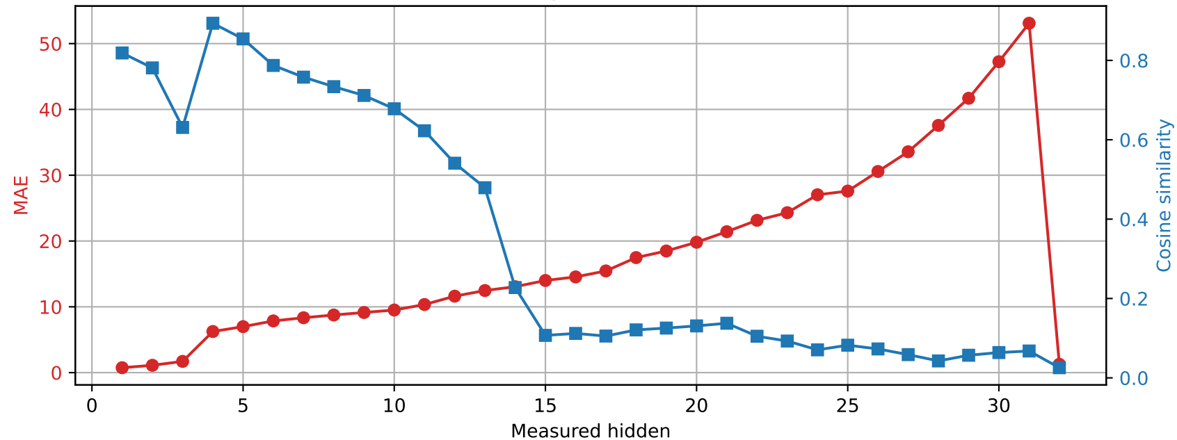
SmolLM2-360M | Prompt 1 Spared layer 24 | Unquantized vs hybrid
