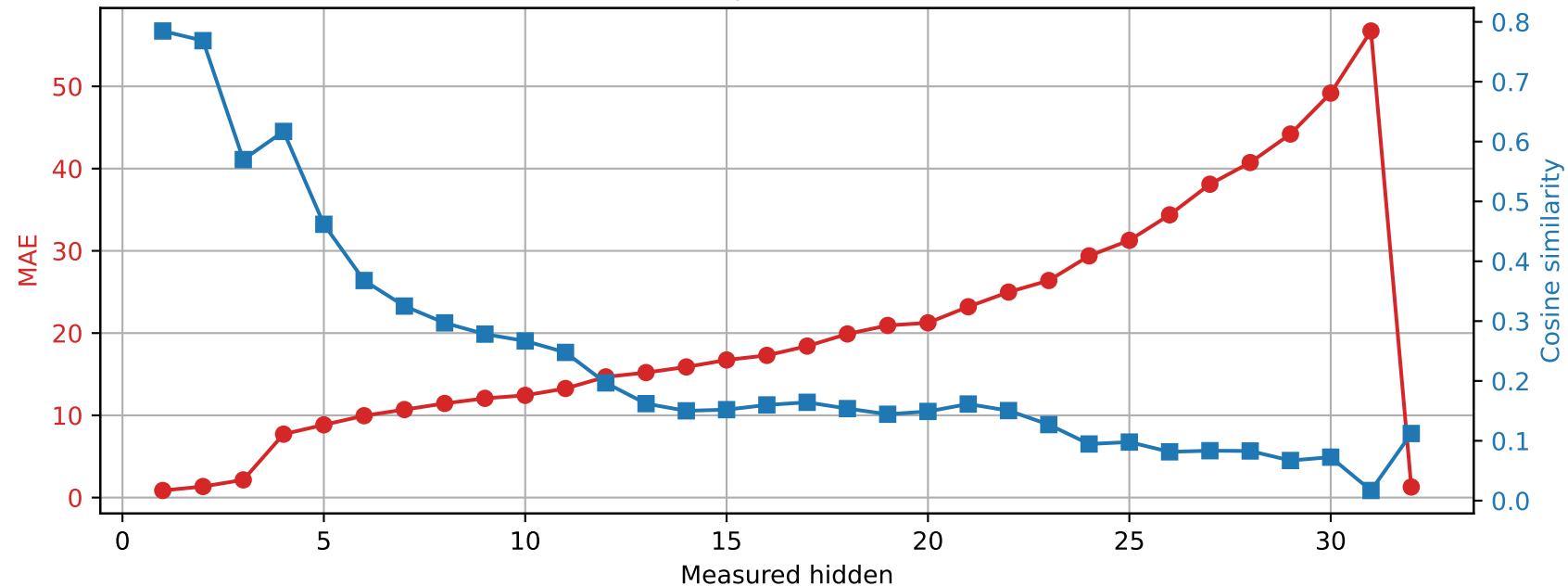
SmolLM2-360M | Prompt 2 Spared layer 19 | Unquantized vs hybrid
