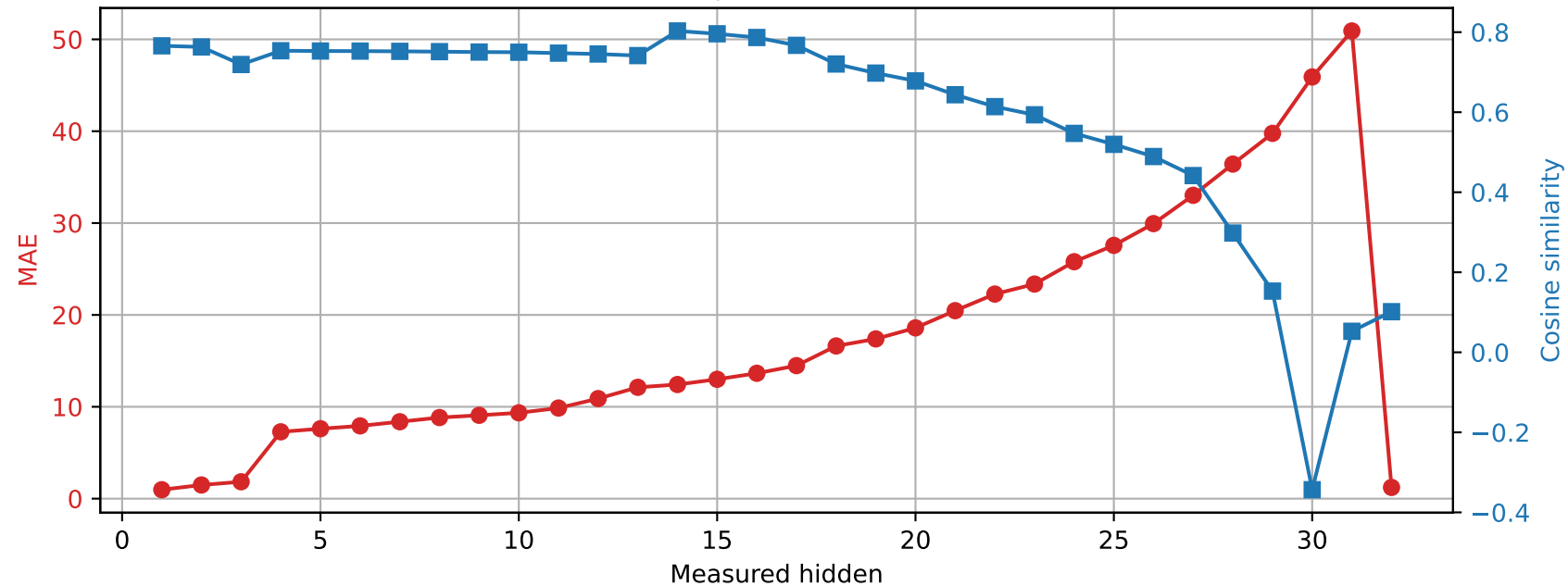
SmolLM2-360M | Prompt 3 Spared layer 2 | Unquantized vs hybrid
