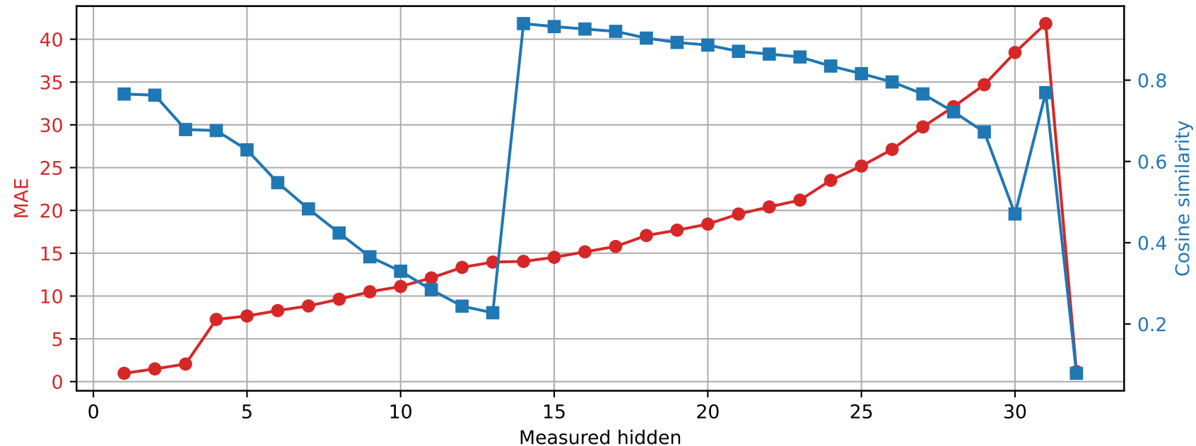
SmolLM2-360M | Prompt 3 Spared layer 3 | Unquantized vs hybrid
