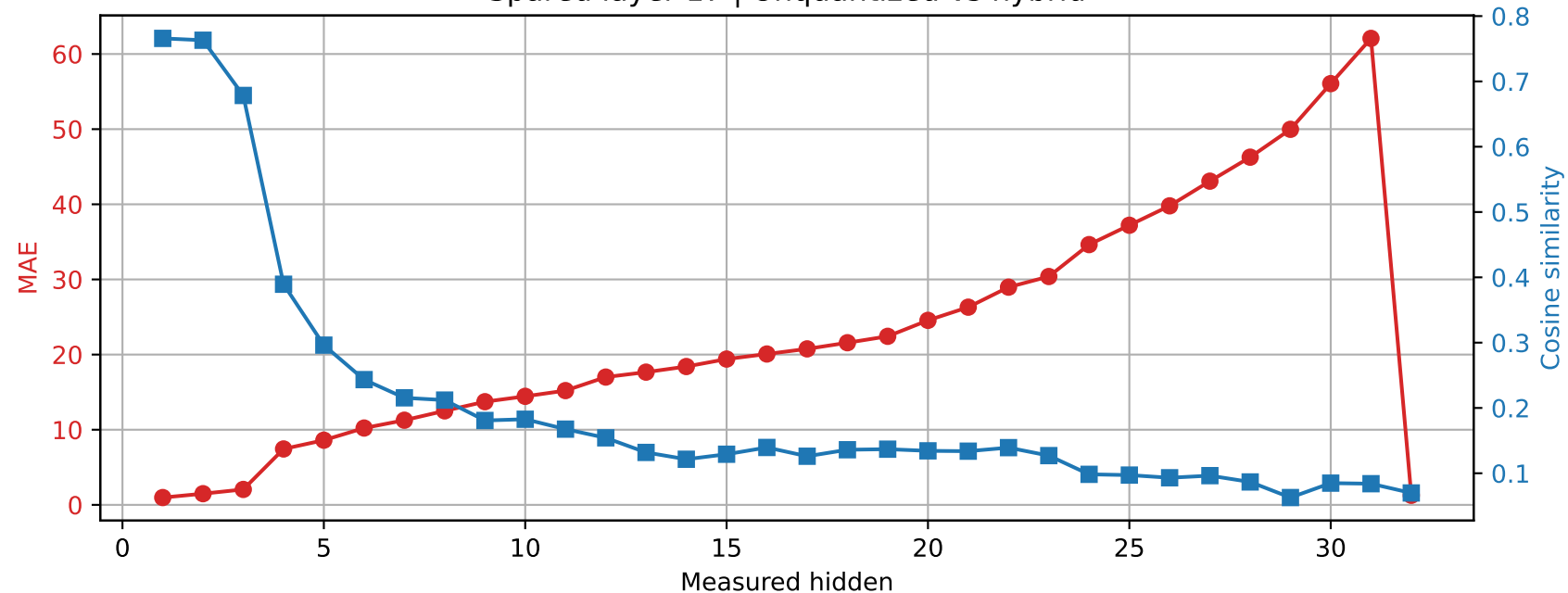
SmolLM2-360M | Prompt 3 Spared layer 17 | Unquantized vs hybrid
