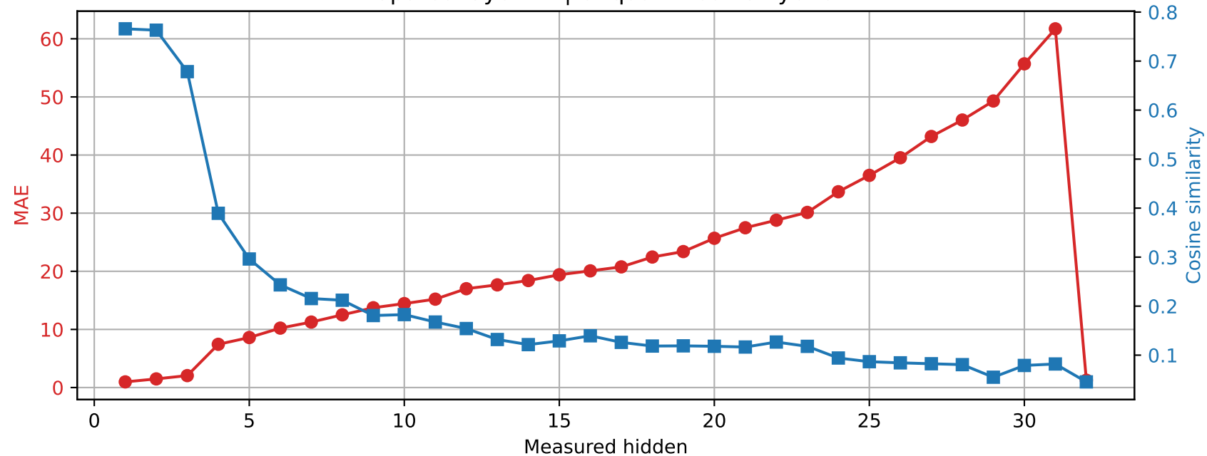
SmolLM2-360M | Prompt 3 Spared layer 21 | Unquantized vs hybrid
