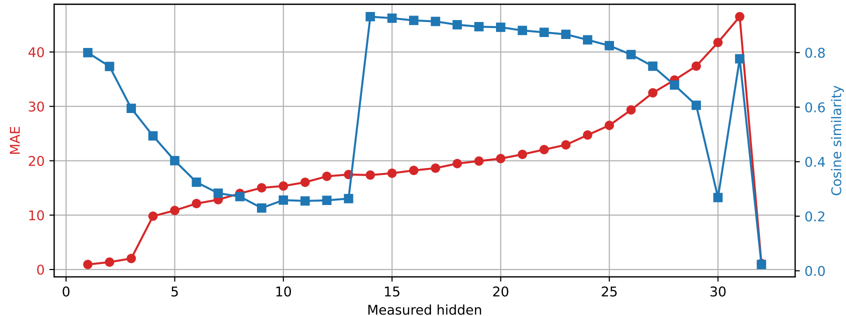
SmolLM2-360M | Prompt 4 Unquantized vs quantized int4
