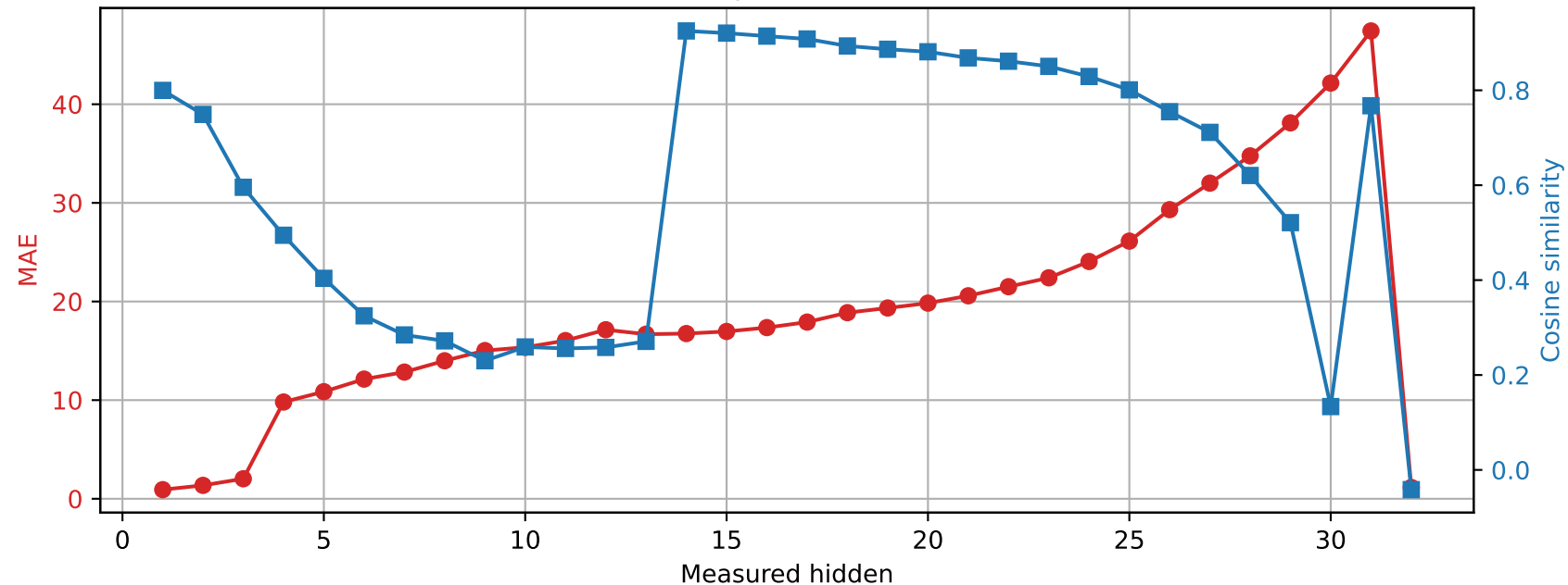
SmolLM2-360M | Prompt 4 Spared layer 12 | Unquantized vs hybrid
