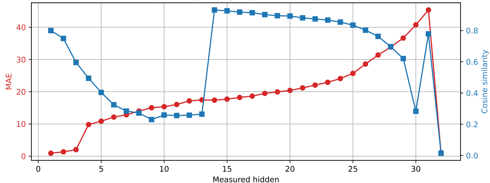
SmolLM2-360M | Prompt 4 Spared layer 23 | Unquantized vs hybrid
