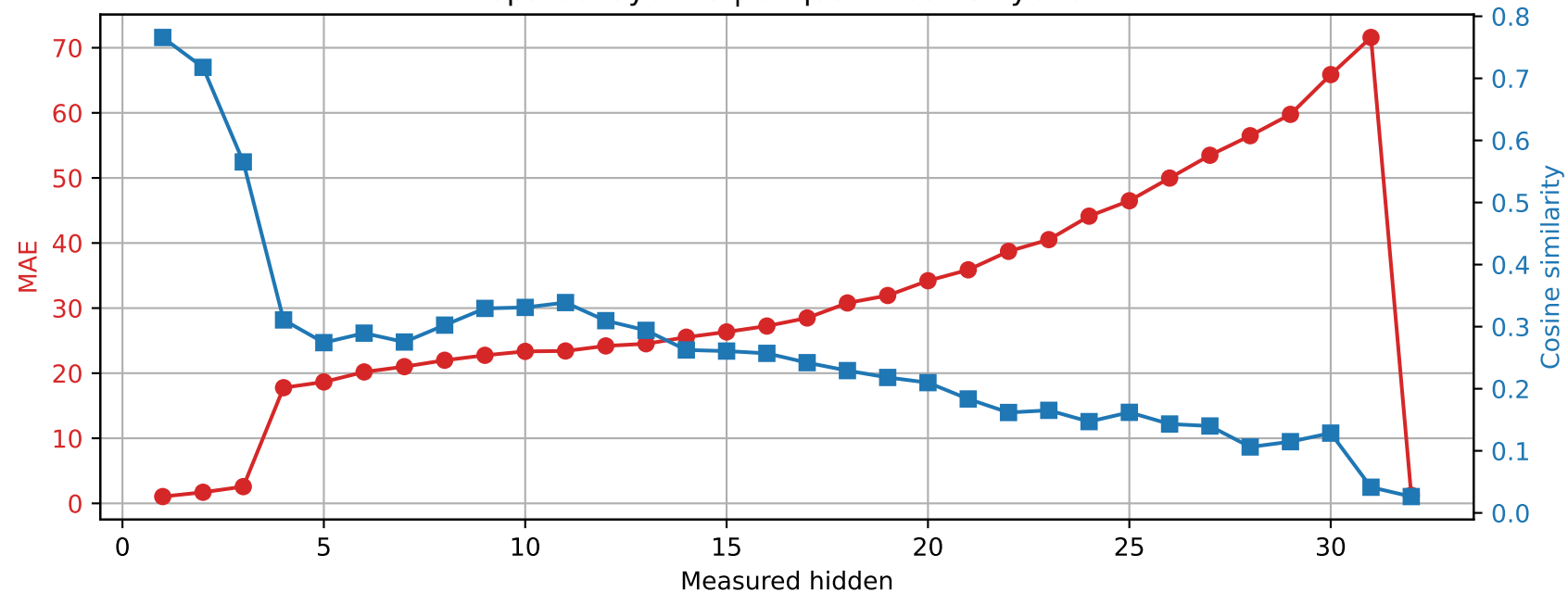
SmolLM2-360M | Prompt 0 Spared layer 10 | Unquantized vs hybrid
