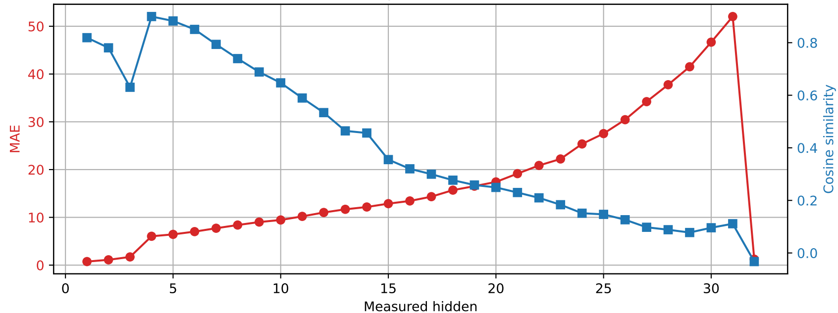
SmolLM2-360M | Prompt 1 Spared layer 3 | Unquantized vs hybrid
