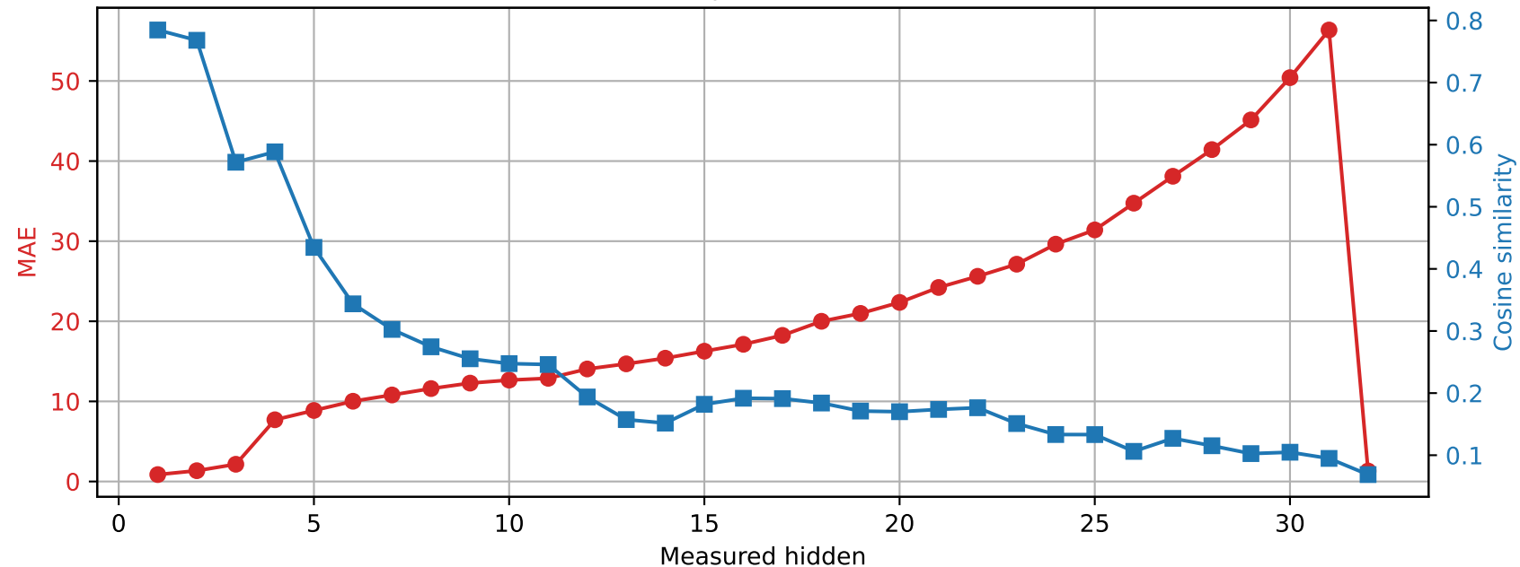
SmolLM2-360M | Prompt 2 Spared layer 10 | Unquantized vs hybrid
