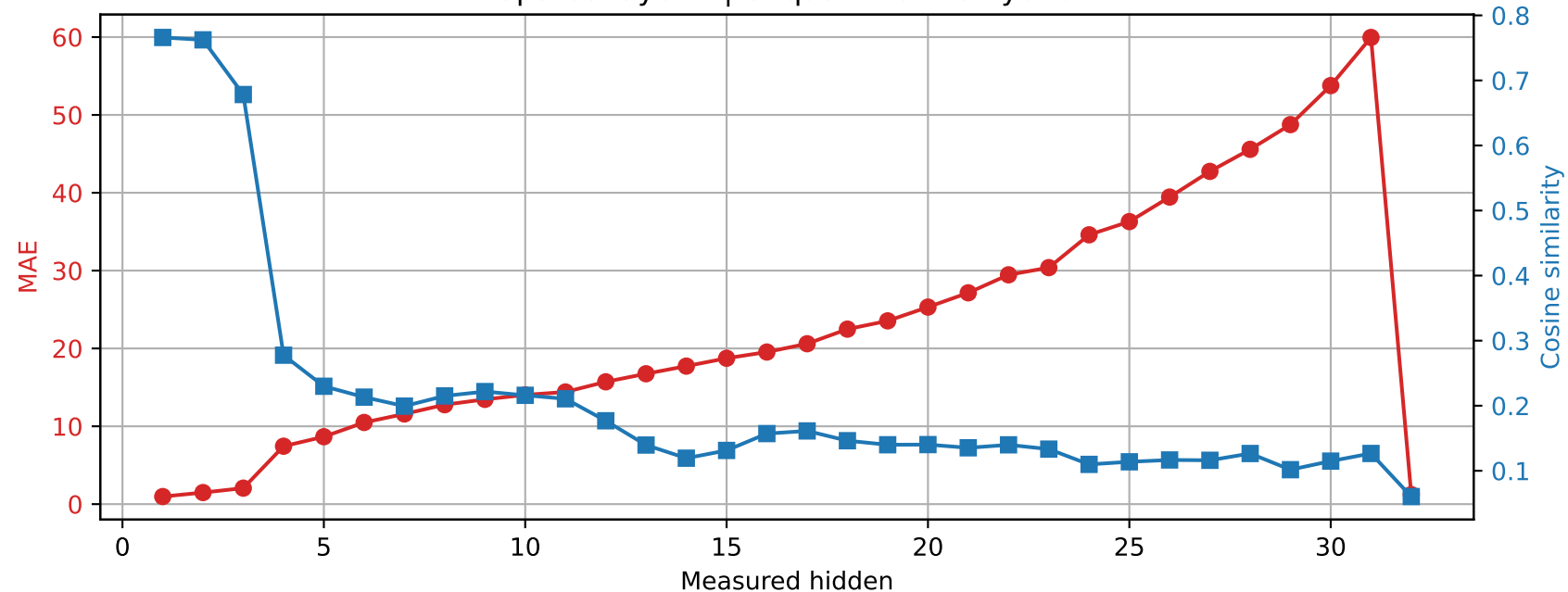
SmolLM2-360M | Prompt 3 Spared layer 7 | Unquantized vs hybrid
