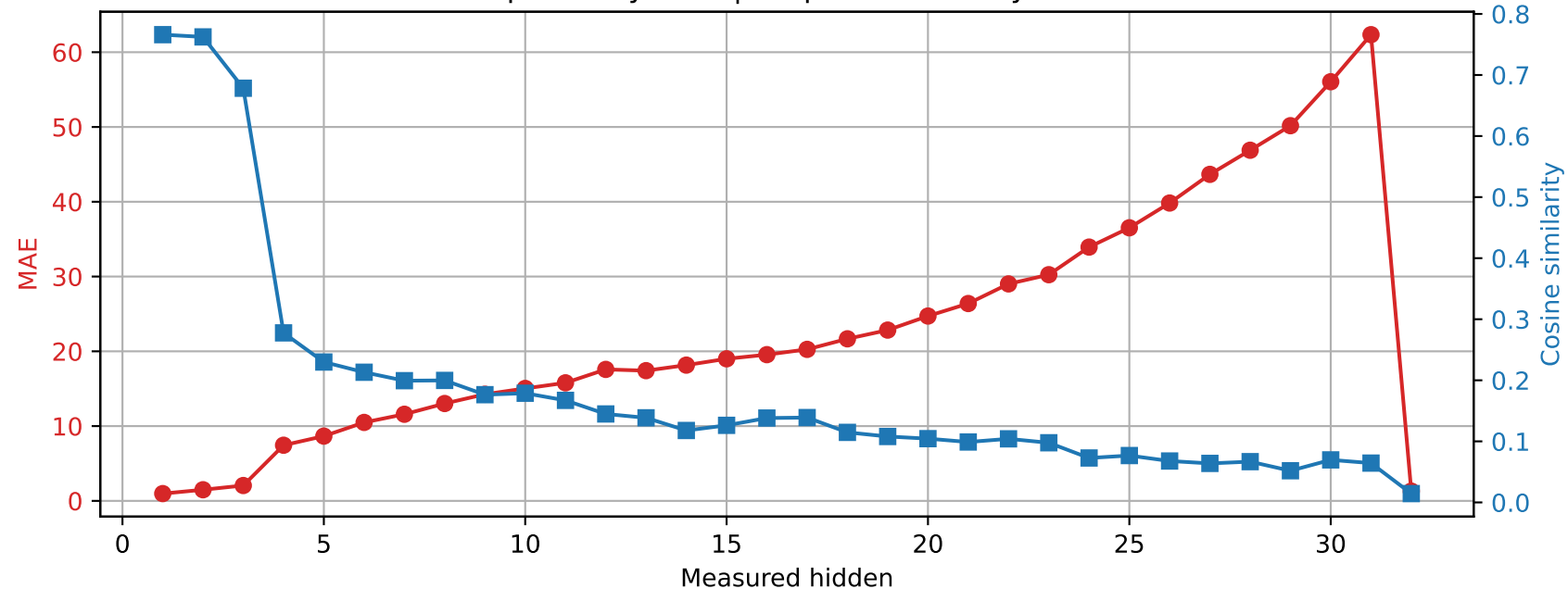
SmolLM2-360M | Prompt 3 Spared layer 12 | Unquantized vs hybrid
