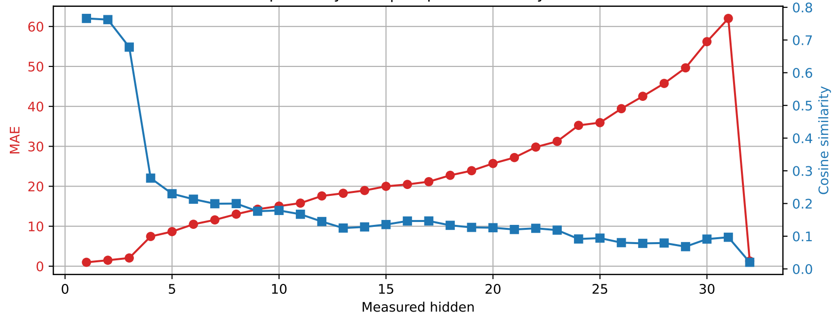
SmolLM2-360M | Prompt 3 Spared layer 24 | Unquantized vs hybrid
