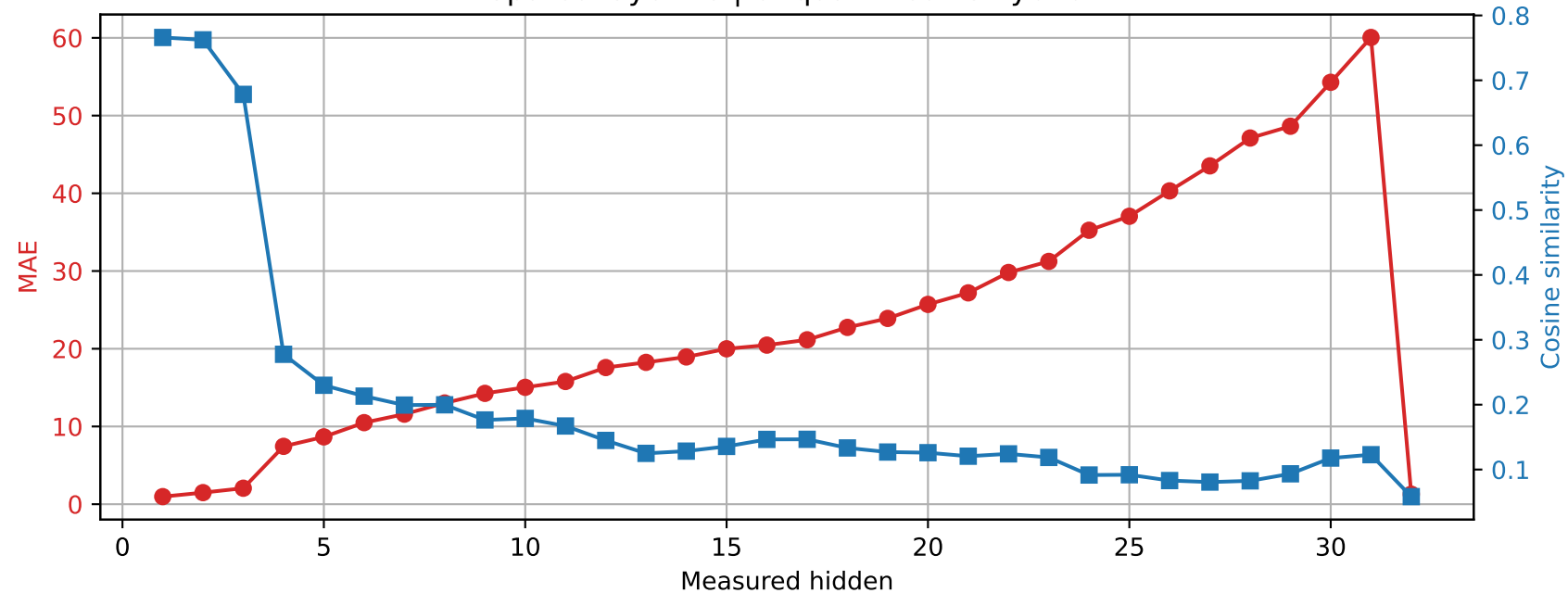
SmolLM2-360M | Prompt 3 Spared layer 28 | Unquantized vs hybrid
