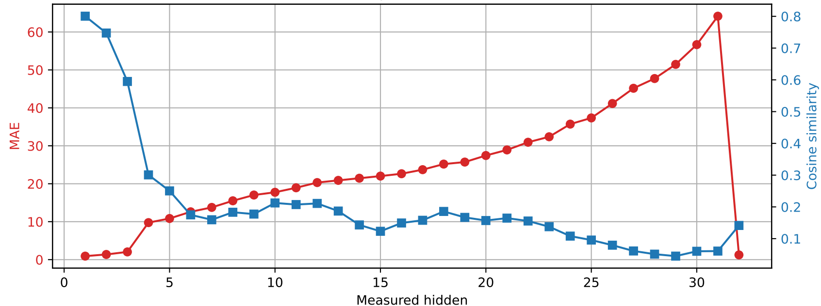
SmolLM2-360M | Prompt 4 Spared layer 3 | Unquantized vs hybrid
