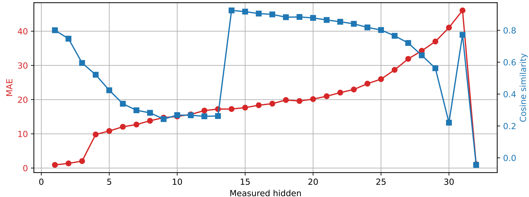
SmolLM2-360M | Prompt 4 Spared layer 18 | Unquantized vs hybrid
