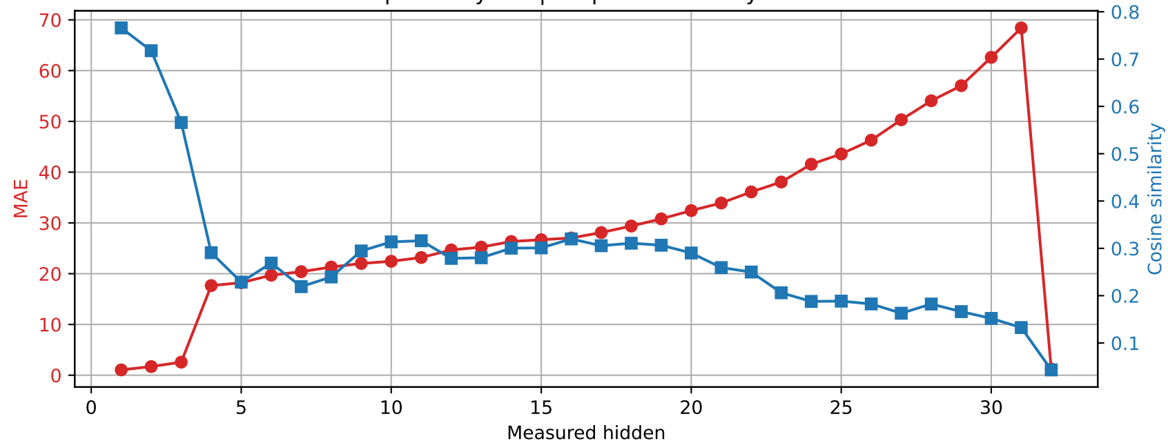
SmolLM2-360M | Prompt 0 Spared layer 3 | Unquantized vs hybrid
