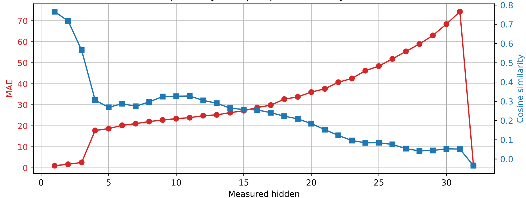
SmolLM2-360M | Prompt 0 Spared layer 15 | Unquantized vs hybrid
