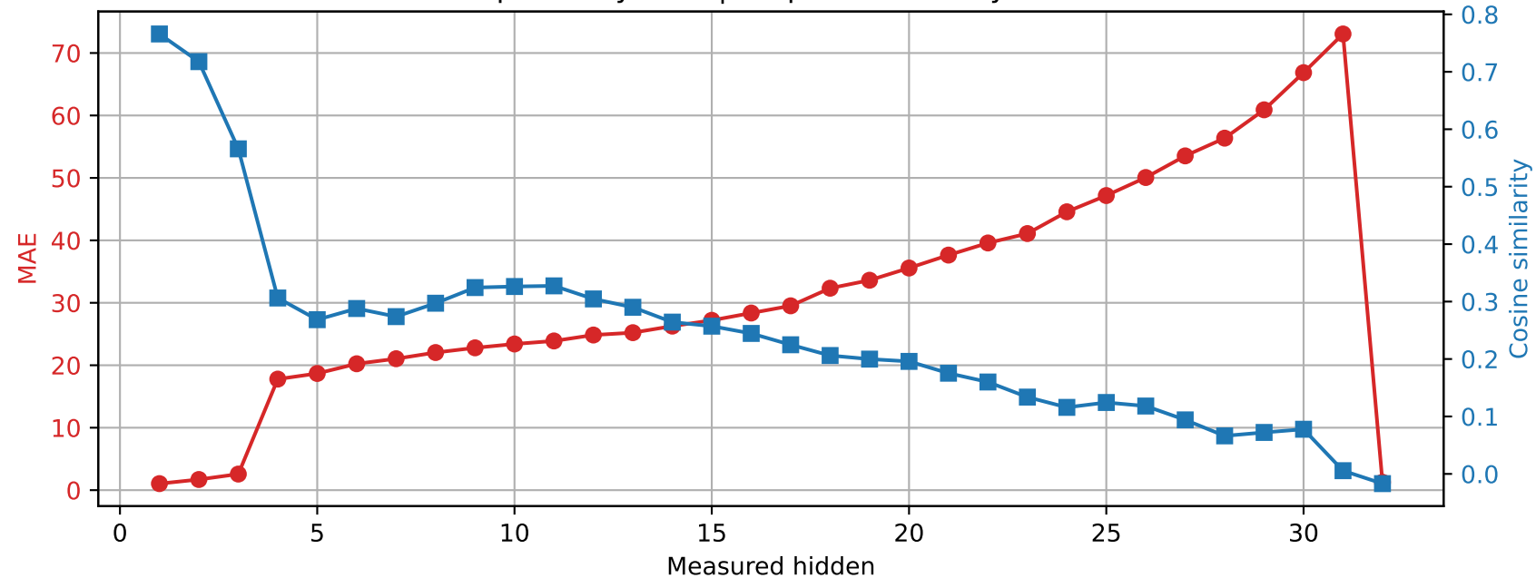
SmolLM2-360M | Prompt 0 Spared layer 21 | Unquantized vs hybrid
