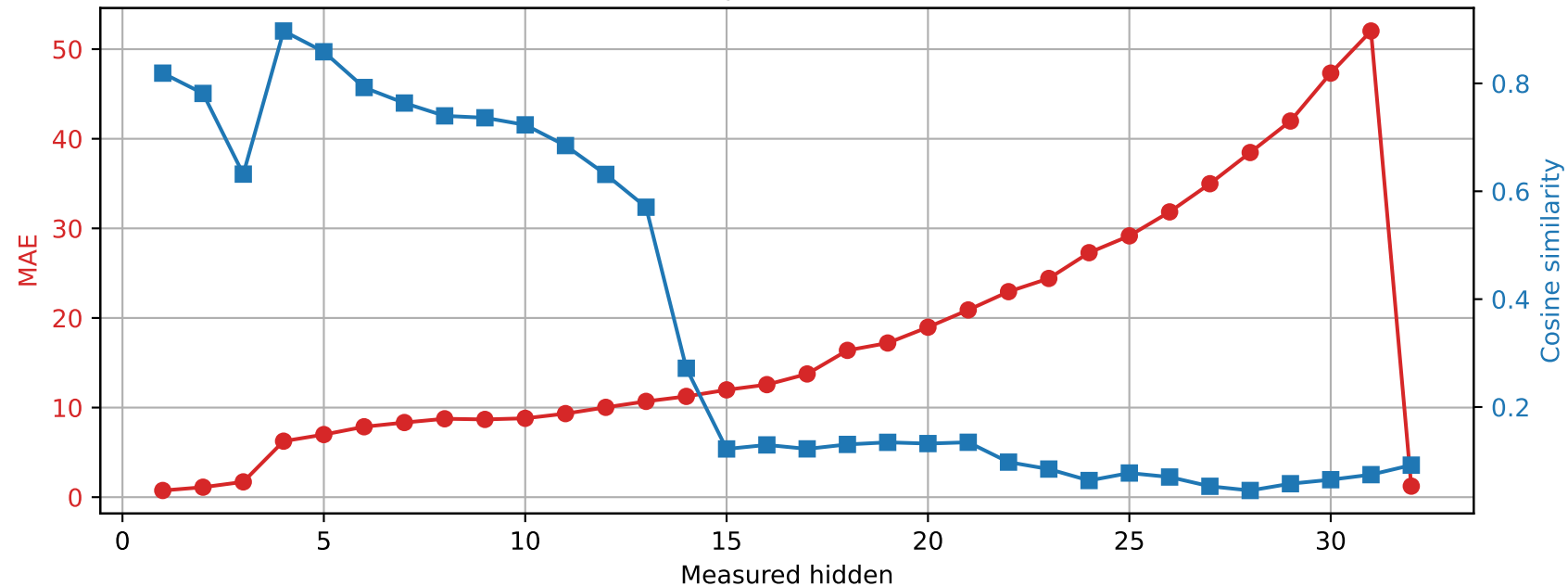
SmolLM2-360M | Prompt 1 Spared layer 8 | Unquantized vs hybrid
