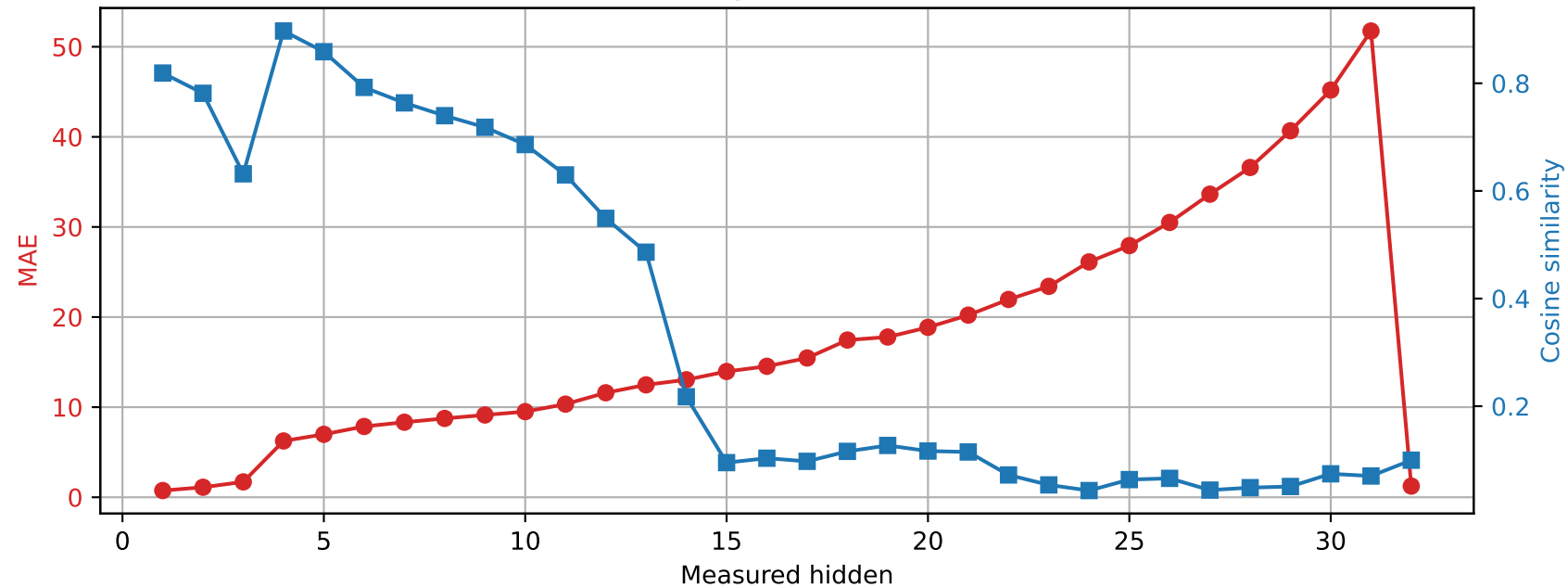
SmolLM2-360M | Prompt 1 Spared layer 18 | Unquantized vs hybrid
