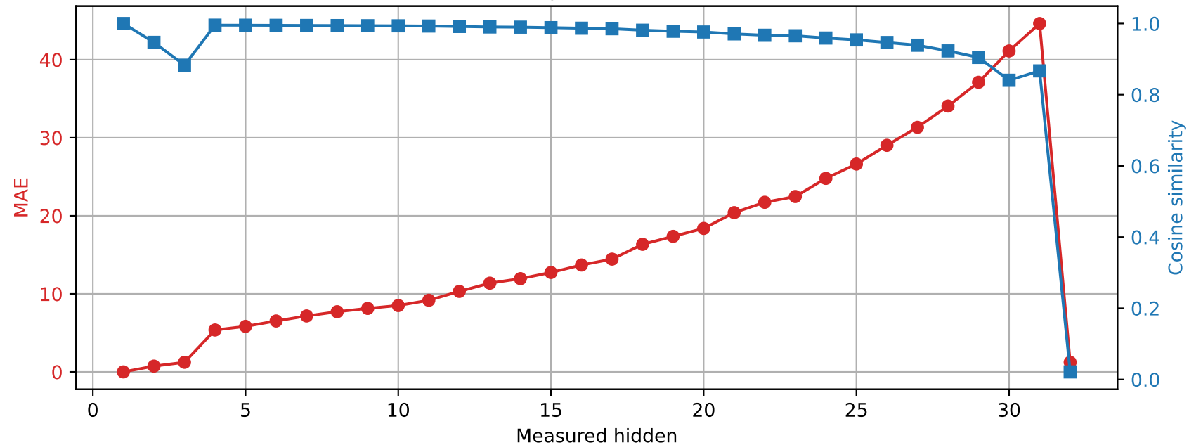
SmolLM2-360M | Prompt 2 Spared layer 0 | Unquantized vs hybrid
