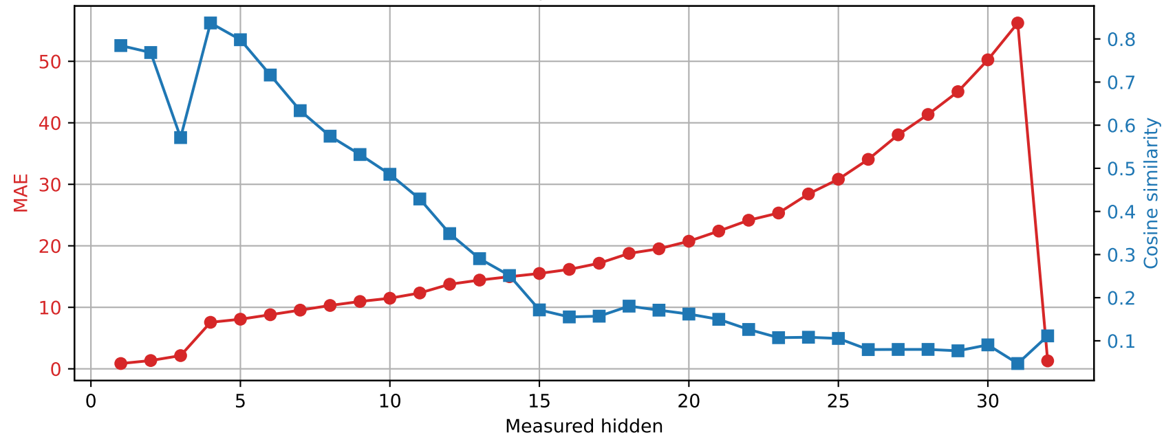
SmolLM2-360M | Prompt 2 Spared layer 3 | Unquantized vs hybrid
