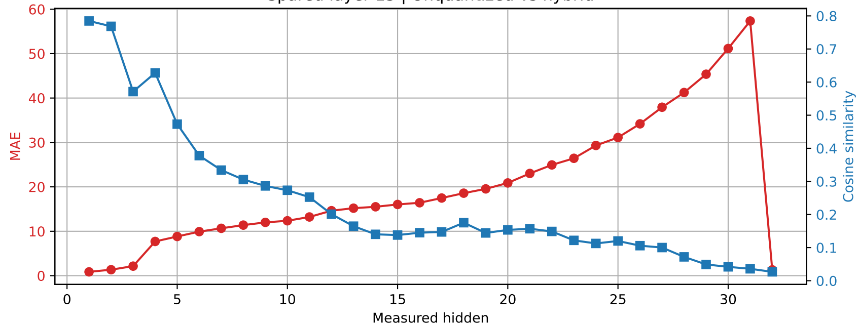
SmolLM2-360M | Prompt 2 Spared layer 13 | Unquantized vs hybrid
