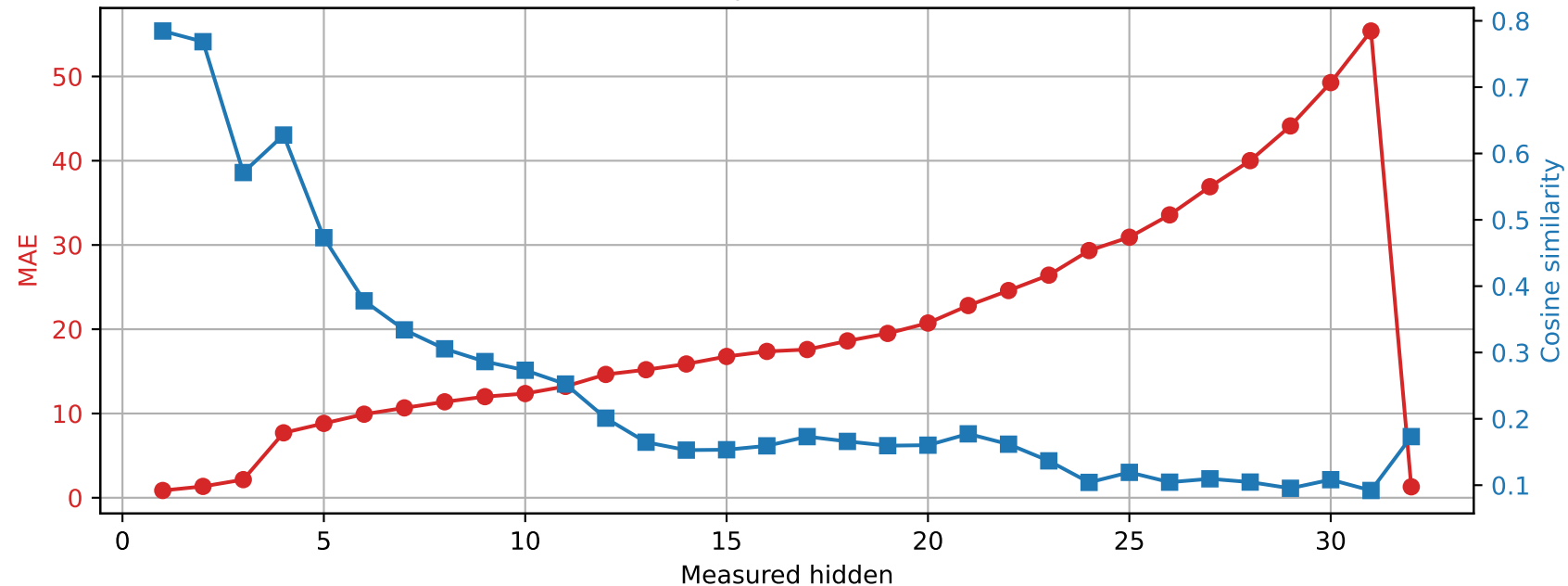
SmolLM2-360M | Prompt 2 Spared layer 16 | Unquantized vs hybrid
