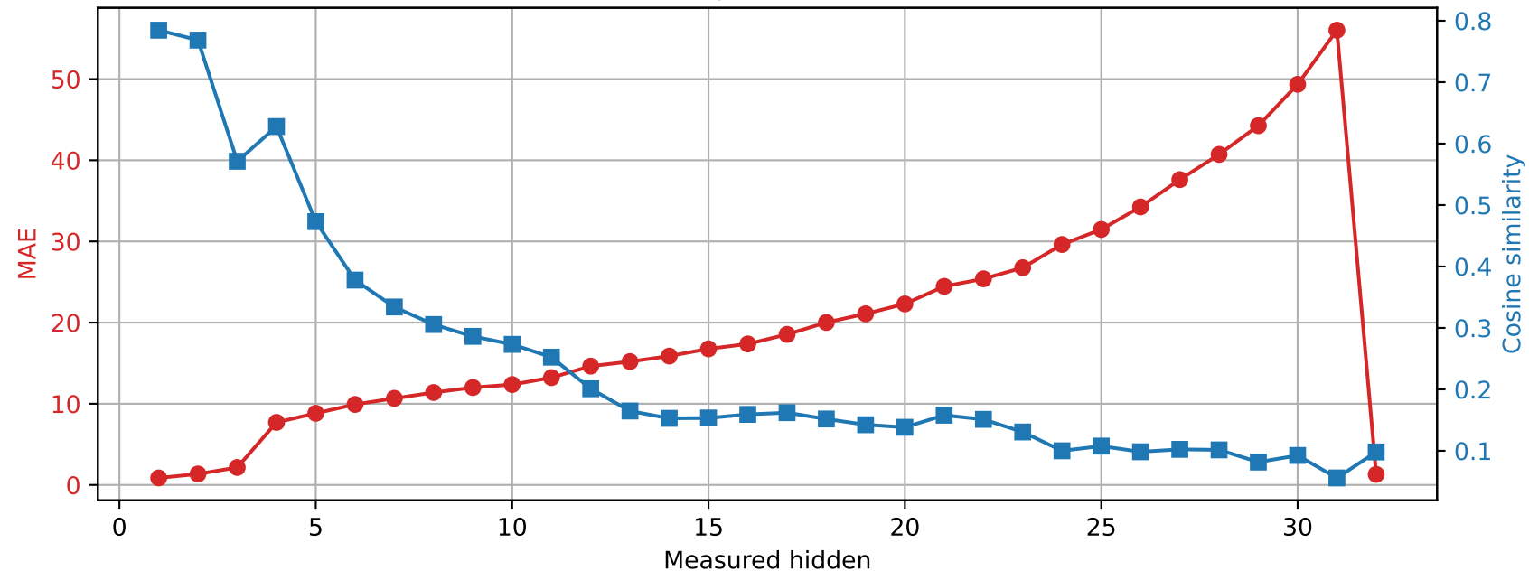
SmolLM2-360M | Prompt 2 Spared layer 21 | Unquantized vs hybrid
