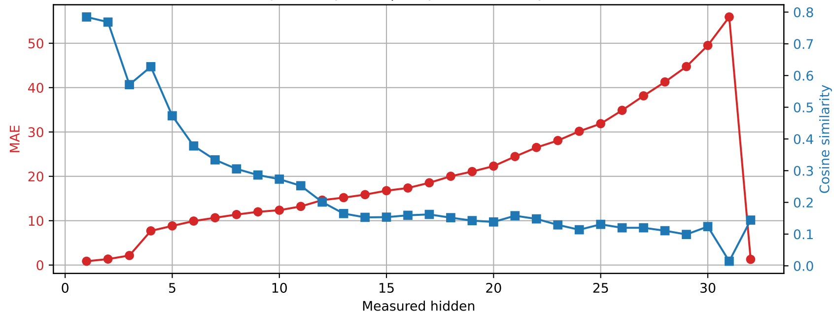
SmolLM2-360M | Prompt 2 Spared layer 23 | Unquantized vs hybrid
