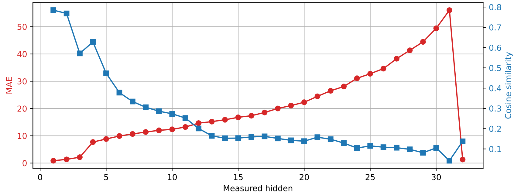
SmolLM2-360M | Prompt 2 Spared layer 25 | Unquantized vs hybrid
